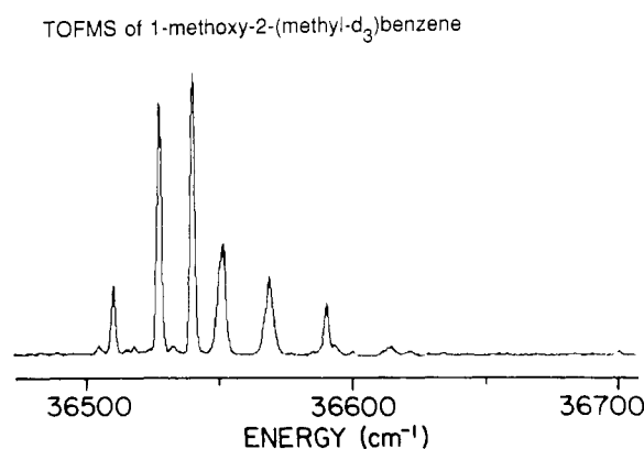
Figure 10. TOFMS of the 0_0^0 region of 1-methoxy-2-(methyl- d_3 )benzene. The origin occurs at 35403.5\text{ cm}^{-1} . The features to the blue of the origin have all shifted closer together upon deuteration than those associated with the protonated compound (Figure 9). Such shifts support the assignment of these features to ring methyl rotational transitions.
