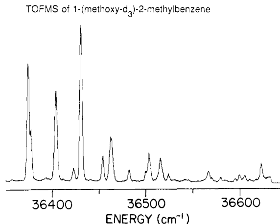
Figure 11. TOFMS of the 0_0^0 region of 1-(methoxy- d_3 )-2-methylbenzene. The origin occurs at 36367.5\text{ cm}^{-1} . The spacings between peaks are the same as in Figure 9. This observation rules out the assignment of any of the observed features as transitions between torsional states of the methoxy group.
