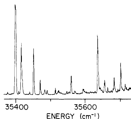
Figure 3. TOFMS of 0_0^0 region of 1-methoxy-4-methylbenzene. The peak at 35400.4\text{ cm}^{-1} is assigned as the origin, while the features at 35417.6 , 35452.7 , and 35484.3\text{ cm}^{-1} are all assigned to internal rotational transitions of the ring methyl group. The intensity displayed by these latter features is unusual and indicates a change in geometry of the methyl group upon excitation from S_0 to S_1 .
