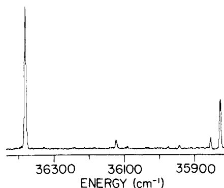
Figure 2. DE spectrum of the 0 0 0 region of methoxybenzene obtained by pumping the 36381.1-cm -1 transition. The spectrum shows a lack of low-lying torsional modes of the methoxy group, as did Figure 1.
