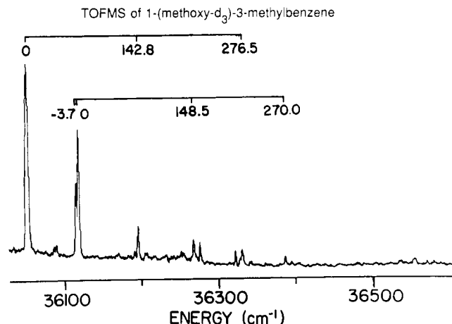
Figure 7. TOFMS of the 0_0^0 region of 1-(methoxy- d_3 )-3-methylbenzene. Deuteriation of the methoxy group has no effect on the spacings of the features in this spectrum relative to those in Figure 5, proving that transitions between internal rotational states of the methoxy group do not appear in the spectrum.
