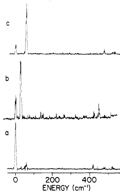
Figure 4. DE spectra of the 0_0^0 region of 1-methoxy-4-methylbenzene obtained by pumping the transitions in Figure 3 at (a) 35400.4 , (b) 35417.6 , and (c) 35452.7\text{ cm}^{-1} . The spacings of the peaks in the spectra enable characterization of the ground-state potential for internal rotation of the ring methyl group.
