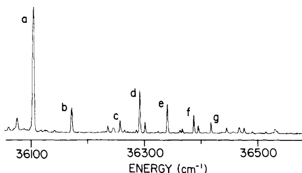
Figure 17. TOFMS of 1,3-dimethoxybenzene for the 0_0^0 region of S_1 \leftarrow S_0 . The peaks labeled a, b, and c occur at 36101.5, 36163.9, and 36256.9 \text{cm}^{-1} and are assigned as origins based on the DE results in Figure 18. The peaks labeled d–g are vibronic features, presumably due to methoxy torsions, built on origin “a”.
