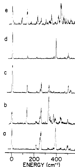
Figure 12. DE spectra of the 0_0^0 region of S_0 \leftarrow S_1 for 1-methoxy-2-methylbenzene, obtained by pumping the transitions labeled a-e in Figure 9. The absence of features within the first 100 cm -1 of the origins indicates that the ring methyl rotor experiences a large ( >200 cm -1 ) barrier to rotation in S_0 .
