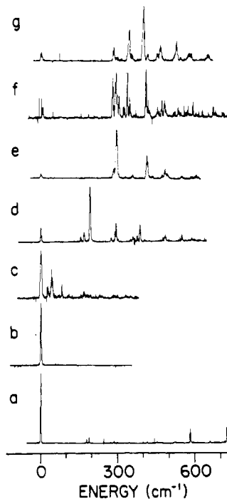
Figure 18. DE spectra of the 0_0^0 region of S_0 \leftarrow S_1 for 1,3-dimethoxybenzene obtained by pumping the transitions labeled a–g in Figure 17. The uniqueness of spectra a–c in this figure lead to the assignment of peaks a–c in Figure 17 as separate origins. The lack of intensity at the origins of spectra d–g, plus their similarities with each other and with “a” lead to the assignments of features d–g in Figure 17 as methoxy torsions built on the origin “a”.
