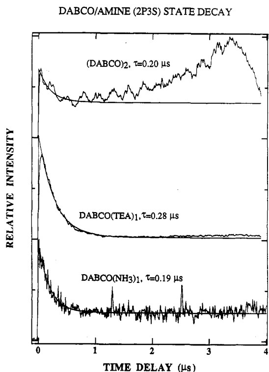
Figure 7. Decay of DABCO/amine cluster (2p3s) Rydberg state observed through origin excitation. The ionization energy is 22 222 cm -1 . Note that the decays end in a constant signal for each case. These curves have been fit to single exponential function plus a constant. The constant signal is assigned as due to long-lived charge-transfer intermediate. The signal rise at later time is probably due to solvent reorganization accompanied by an ionization efficiency enhancement.
