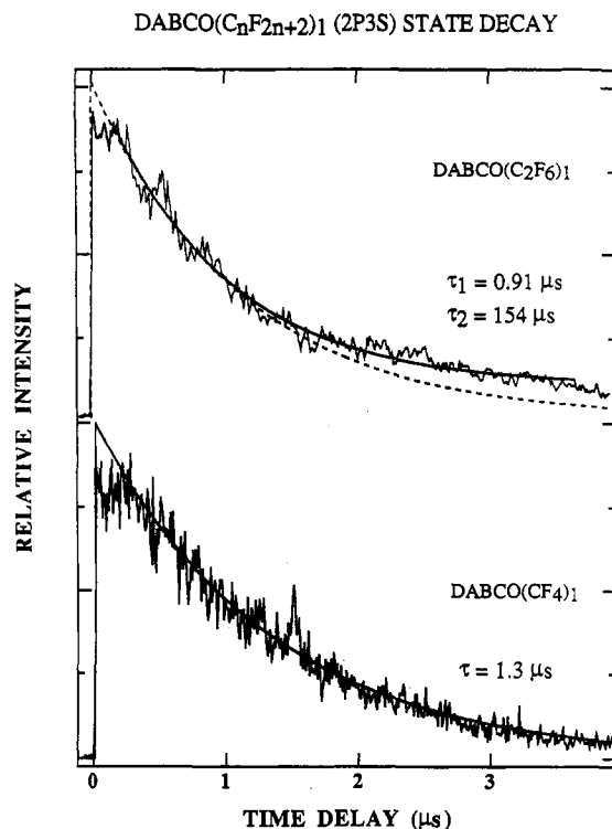
Figure 6. Decay of DABCO/perfluorocarbon cluster (2p3s) singlet Rydberg states. The ionization energy is 22 222 cm -1 . Both clusters are excited at their origin transitions (36 206 cm -1 for (CF 4 ) 1 and 36 090 cm -1 for (C 2 F 6 ) 1 clusters). The DABCO(CF 4 ) 1 decay is fit to a single exponential function with a lifetime of 1.3 μs. The DABCO(C 2 F 6 ) 1 decay curve is best fit by a biexponential decay function (solid line); a single exponential decay function (dashed line) generates a poor fit.
