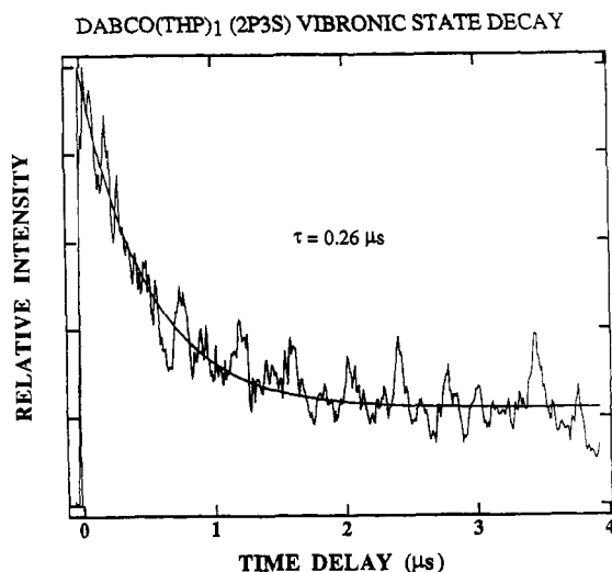
Figure 10. Decay of DABCO(THP) 1 excited at 36 898 cm -1 ( 0^0 + 1665 \text{ cm}^{-1} ). The ionization energy is 22 222 cm -1 . Note the signal does not approach zero at long times. The decay curve can be fit to a single exponential function plus a constant. This result indicates that the DABCO(THP) 1 cluster does not dissociate in the new state.
