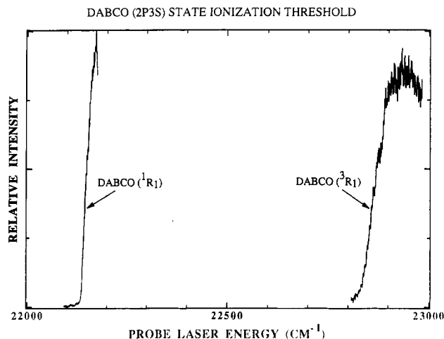
Figure 4. Photoionization threshold spectra of the excited singlet and triplet Rydberg states of DABCO. The singlet excited state ( ^1R_1 ) ionization curve is obtained by excitation of DABCO at its vibronic transition peak at 36\,477\text{ cm}^{-1} . The triplet Rydberg state ( ^3R_1 ) ionization curve is obtained by excitation of the DABCO(Kr); “geometry II” cluster transition at 36\,075\text{ cm}^{-1} , while monitoring the DABCO ion mass channel with the ionization laser delayed 3\text{ }\mu\text{s} with respect to the excitation laser. The ionization energies for ^1R_1 and ^3R_1 states are 22\,137 and 22\,830\text{ cm}^{-1} , respectively.
