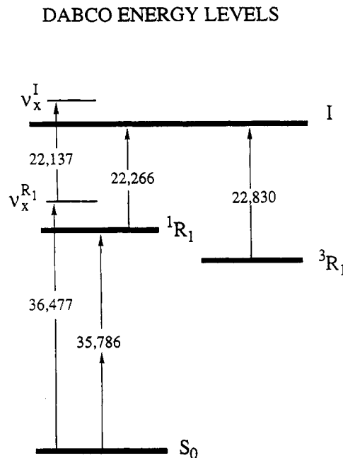
Figure 5. Experimentally determined energy level diagram of the DABCO bare molecule ( \text{cm}^{-1} ). The value for the ^1\text{R}_1\ 0^0 ionization energy is obtained from the reported total ionization energy ( 58\ 052\ \text{cm}^{-1} ) minus the excitation energy.
