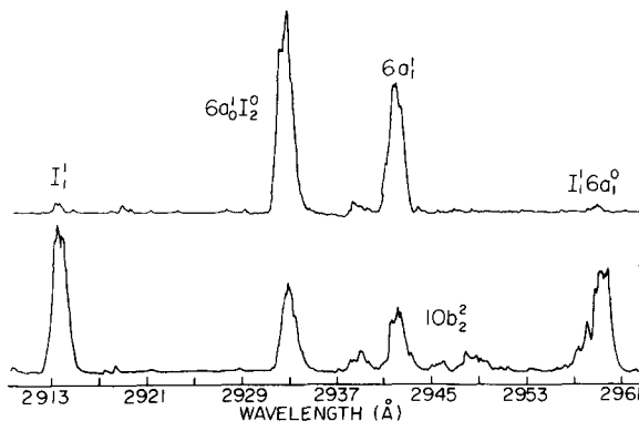
FIG. 4. DE spectra of \text{An} 6a_1^1 . The upper trace is obtained from \text{An-He} with 0.2\% \text{ CH}_4 expanded at P_0=500 psi. The lower spectrum was obtained from \text{An} expanded with pure \text{He} at P_0=600 psi. Notice the dramatic decrease in the relaxed peaks, particularly I_1^1 and I_1^1 6a_1^0 due to the addition of \text{CH}_4 .
