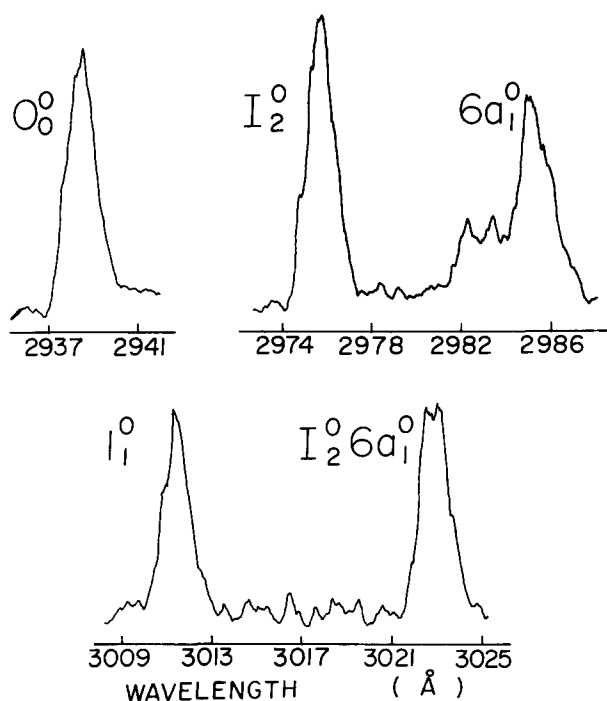
FIG. 17. Portions of the DE spectrum of \text{AnCH}_4 15_2^0 . An was expanded in He with 0.1% \text{CH}_4 at P_0 = 600 psi. The observed \text{AnCH}_4 15_2^0 emission is identical to \text{An} 0_0^0 emission indicating complete and rapid VP at 15_2^0 of \text{AnCH}_4 .
