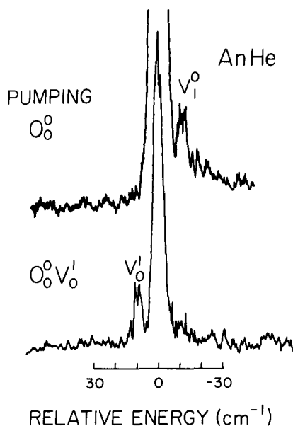
FIG. 3. One of the DE peaks obtained by pumping \text{AnHe} 0_0^0 (upper trace) and one quantum of the \text{AnHe} stretch. \text{An} was expanded with pure \text{He} at P_0=600 psi. The frequency scale is relative to \text{AnHe} 0_0^0 . For these spectra, the slits are reduced to 5 \text{ cm}^{-1} resolution. These spectra confirm the assignments of the absorption features being pumped.
