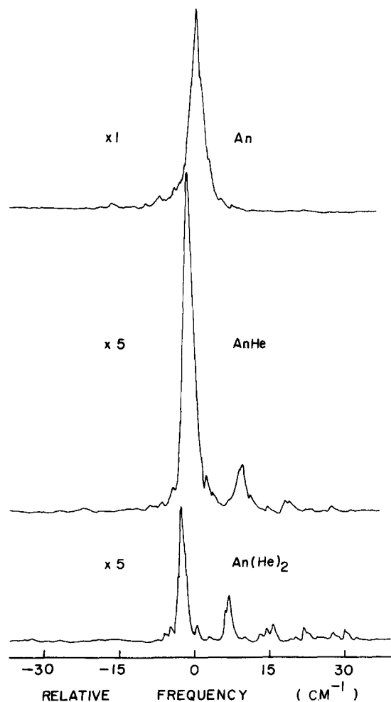
FIG. 2. Two-color MS gated on the labeled species. \text{An} was expanded in pure \text{He} at P_0=600 psi. The frequency scale is relative to \text{An} 0_0^0 . Note that fragmentation has been virtually eliminated. The ionization frequency is 28169 \text{ cm}^{-1} .
