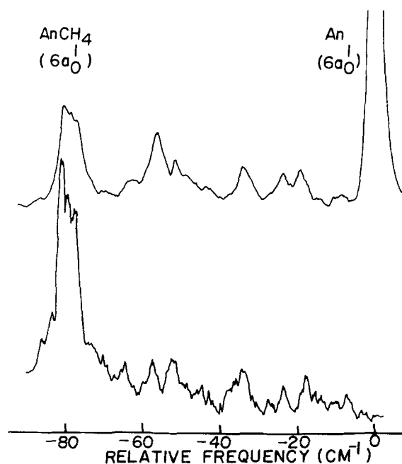
FIG. 12. FE spectrum of An in He with 0.2% \text{CH}_4 at P_0 = 500 psi near the An 6a_0^1 transition (upper trace) and two-color MS of \text{AnCH}_4 for An in He with 0.1% \text{CH}_4 at P_0 = 500 psi and \nu_l = 28219 \text{ cm}^{-1} . Frequency scale is relative to An 6a_0^1 ( 34523 \text{ cm}^{-1} ). Notice that the FE spectrum in this region is due largely to \text{AnCH}_4 .
