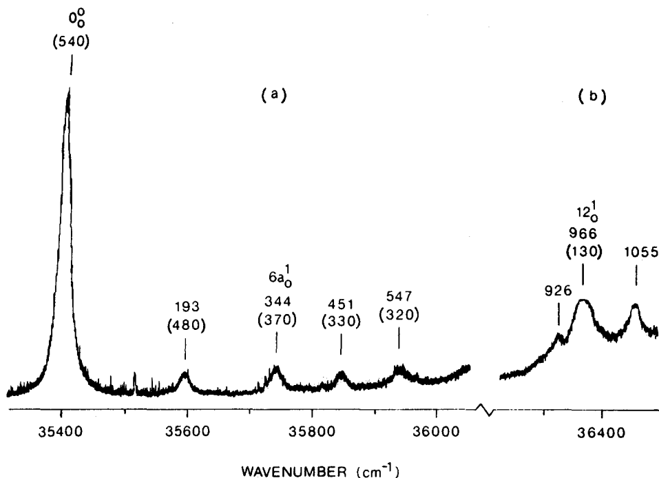
FIG. 1. S_2 \leftarrow S_0 photoexcitation spectrum of acetophenone. The spectra are normalized to the laser intensity. Intensity scales in (a) and (b) are different. In (b), the 12_0^1 band is shown truncated at \sim 85\% of its true peak intensity which is \sim 20\% of the 0_0^0 intensity. Vibronic band positions are indicated relative to the 35\,402\text{ cm}^{-1} 0_0^0 transition. Assignments are given in the figure for some of the features and selected lifetimes are shown in parentheses (in ns). The reported lifetimes are measured in emission by single vibronic level excitation of the vibronic bands indicated. Several weak features appear in the spectrum with narrow ( 2\text{--}3\text{ cm}^{-1} ) linewidths and are assigned to impurities in the sample.
