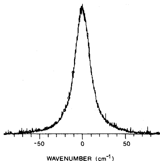
FIG. 2. Expanded view of the acetophenone S_2 0_0^0 observed in photoexcitation. The spectrum is normalized to the laser intensity and displayed relative to the center-line wave number of 35\,402\text{ cm}^{-1} . The open circles in the lower left portion of the band are fit to a Lorentzian line shape with \Gamma = 20.5\text{ cm}^{-1} .
